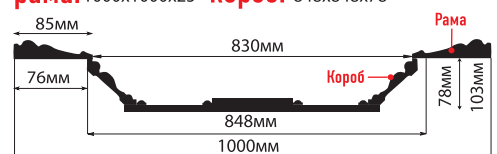
KP100-7D (1000x1000x103)
