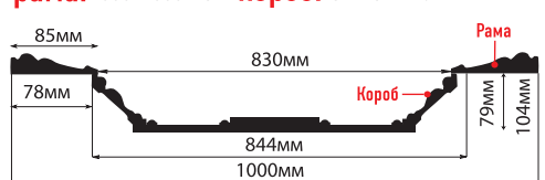
KP100-41 (1000x1000x104)
