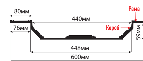
KS61-19D рама: 600x600x12, короб: 448x448x59
