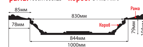
KP100-42 (1000x1000x104)
