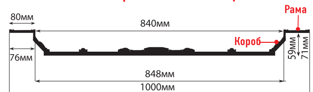
KP100-18D (1000x1000x71) рама: 1000x1000x12 короб: 848x848x59
