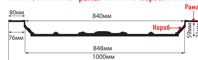
KP100-57 (1000x1000x71) рама: 1000x1000x12 короб: 848x848x59
