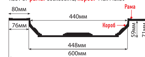
KS61-57 рама: 600x600x12, короб: 448x448x59
