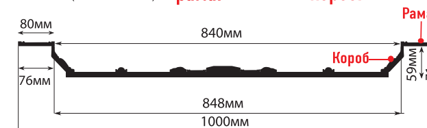
KP100-58 (1000x1000x71)
